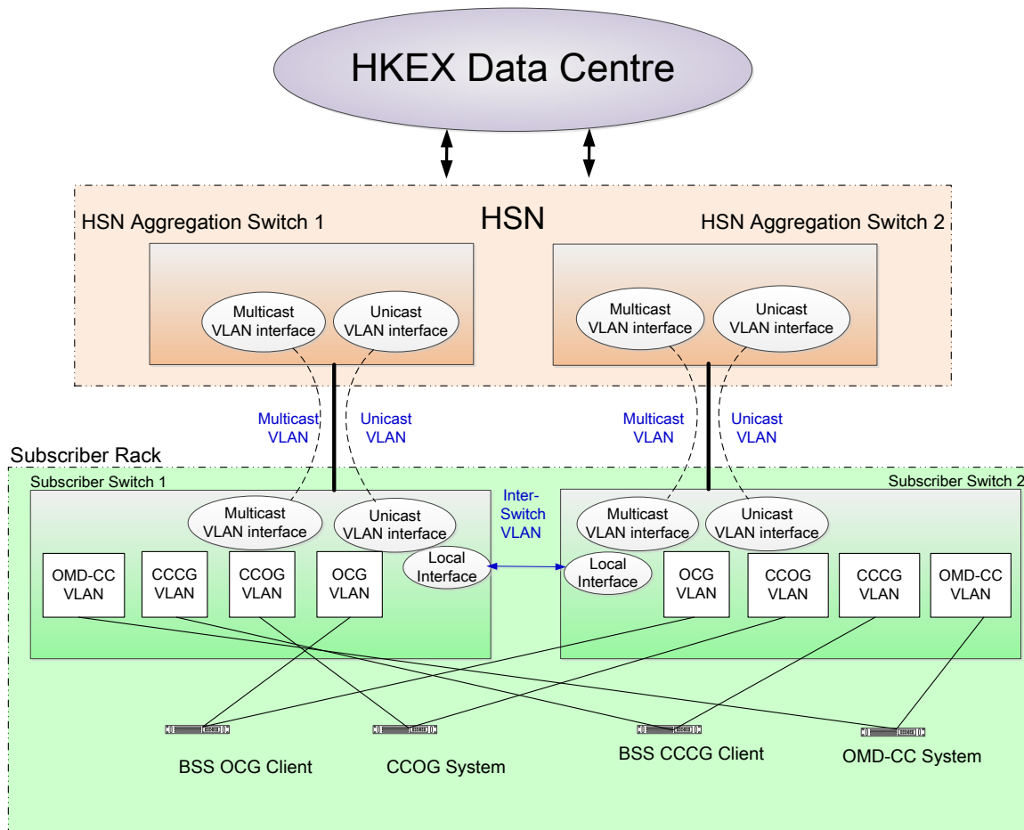
Figure-4 HSN for OCG, CCOG, CCCG and OMD-CC
