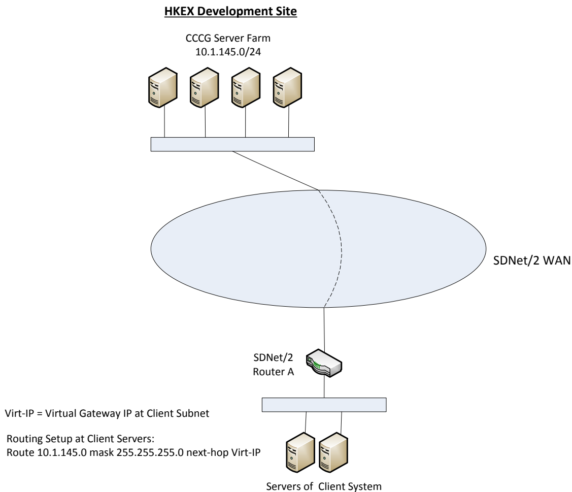
Figure-5 End-to-End Testing Network for CCCG (Single SDNet/2 Circuit)
