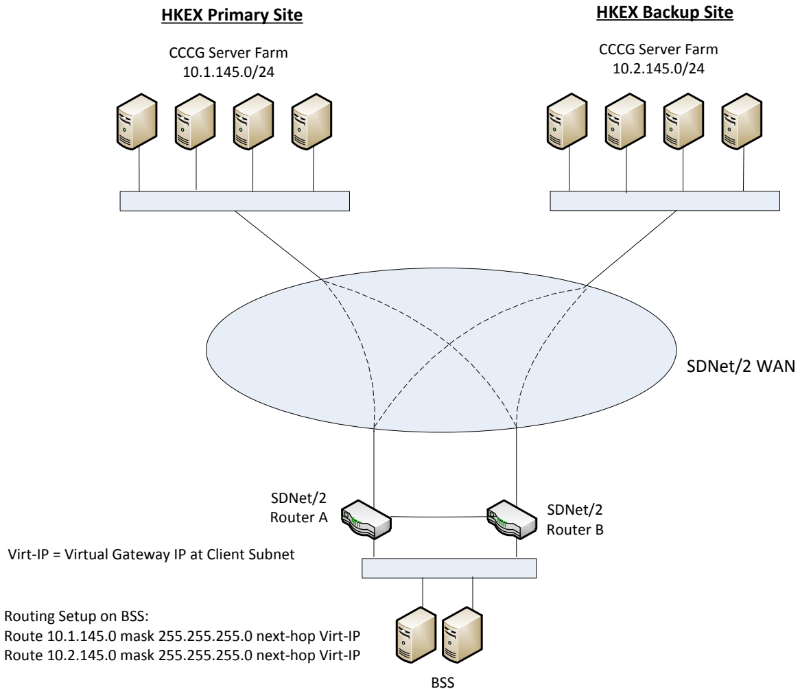
Figure-2 BSS Network Setup for CCCG
