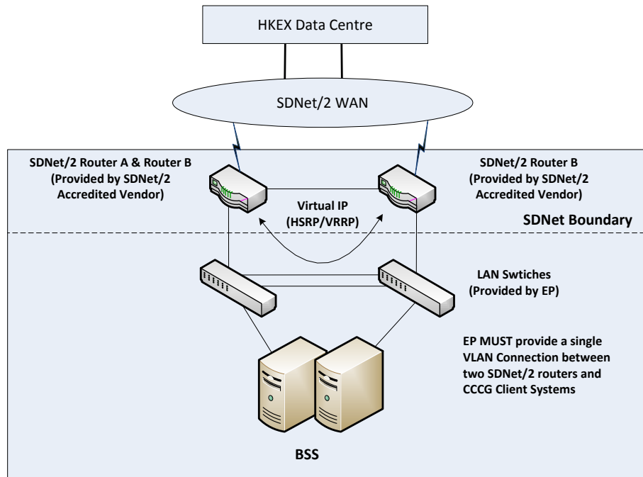
Figure-1 EP Network for CCGG
