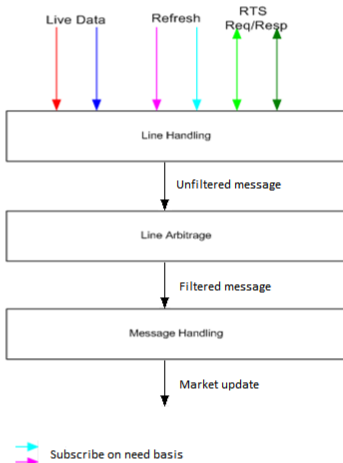
Diagram 1. A Basic Client Application Layout
