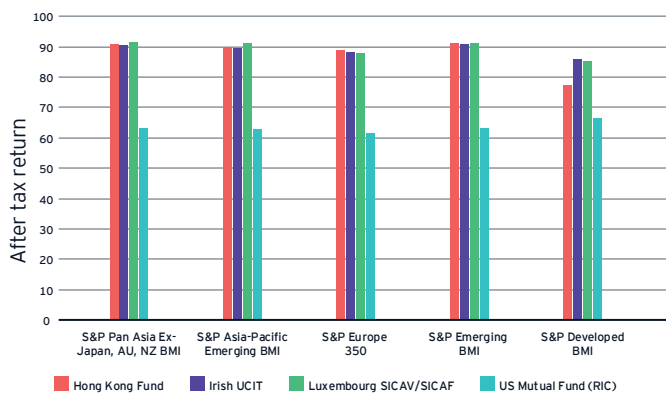
Figure 2. Dividends from indices
