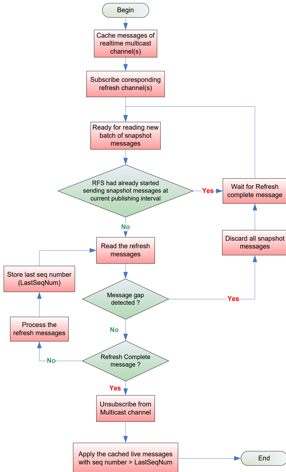
Figure 2. Workflow of Refresh
