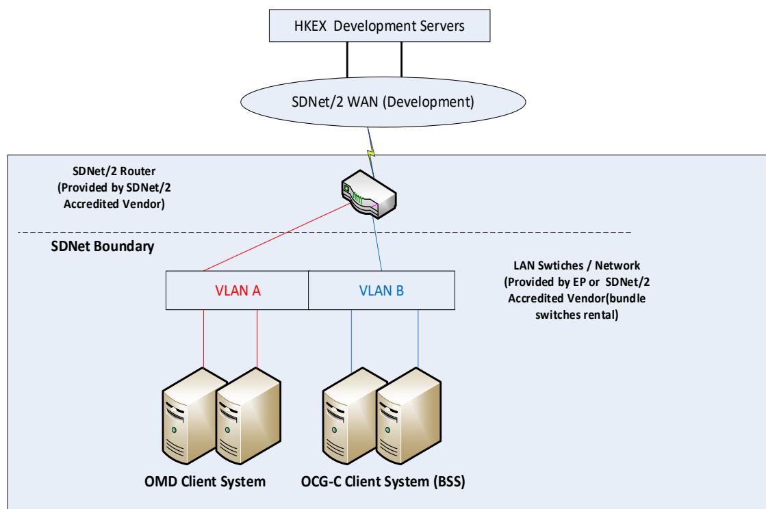
Figure-6 Sharing SDNet/2 Testing Circuit among OCG-C and OMD-C
