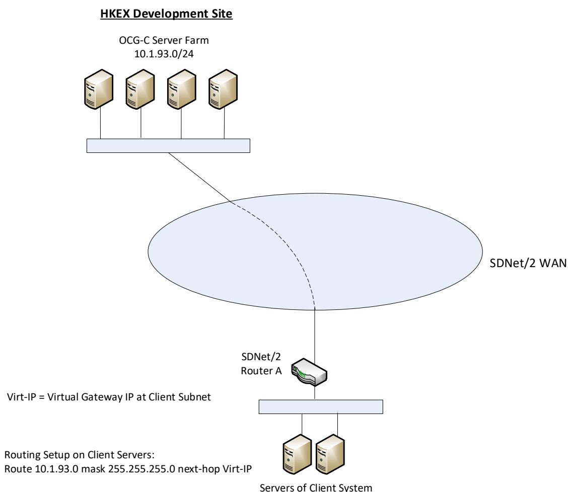
Figure-5 End-to-End Testing Network for OCG-C (Single SDNet/2 Circuit)
