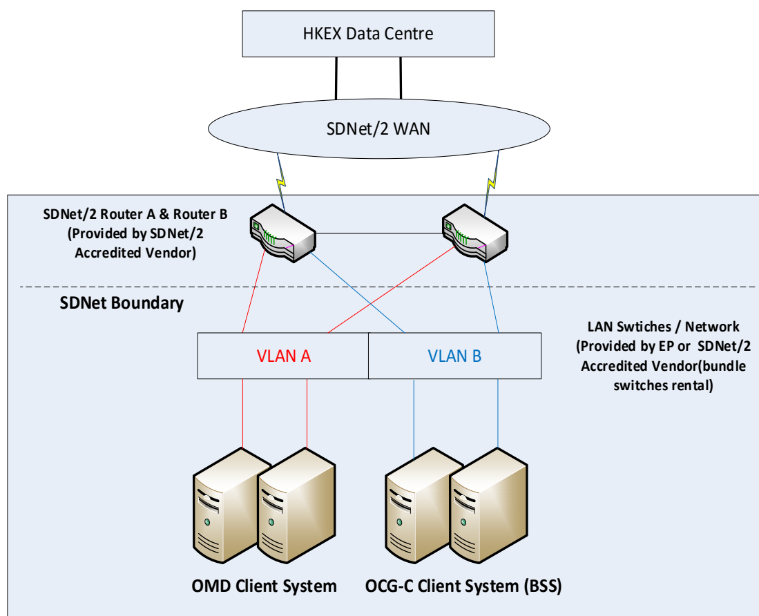
Figure-3 Sharing SDNet/2 Circuit between OCG-C and OMD-C
