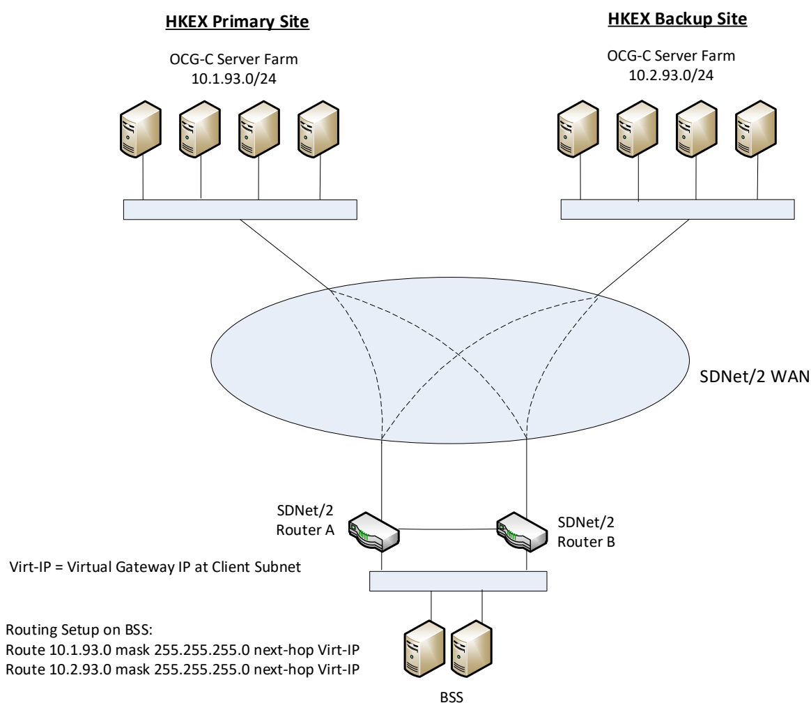
Figure-2 BSS Network Setup for OCG-C
