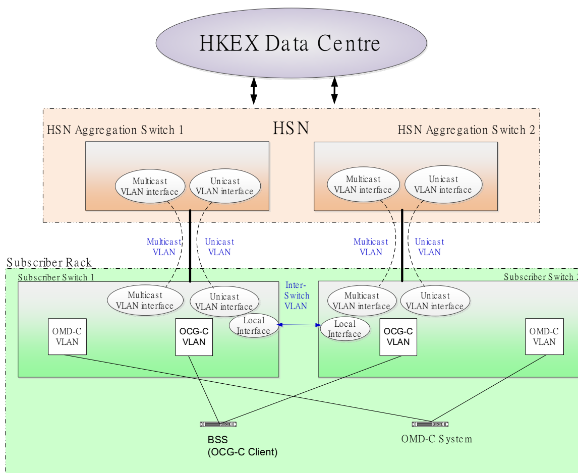
Figure-4 HSN for OCG-C and OMD-C
