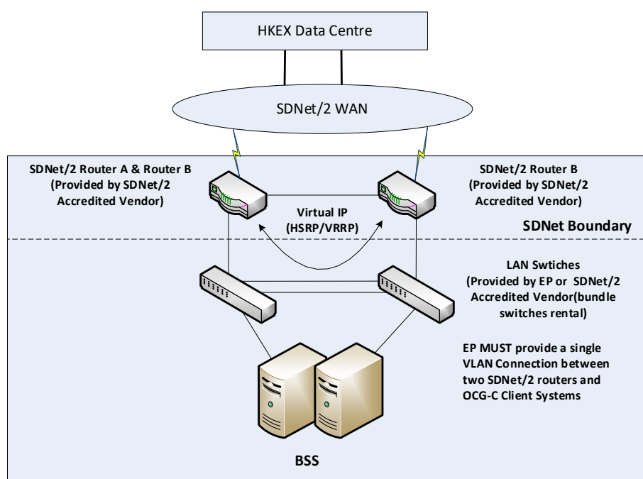
Figure-1 EP Network for OCG-C
